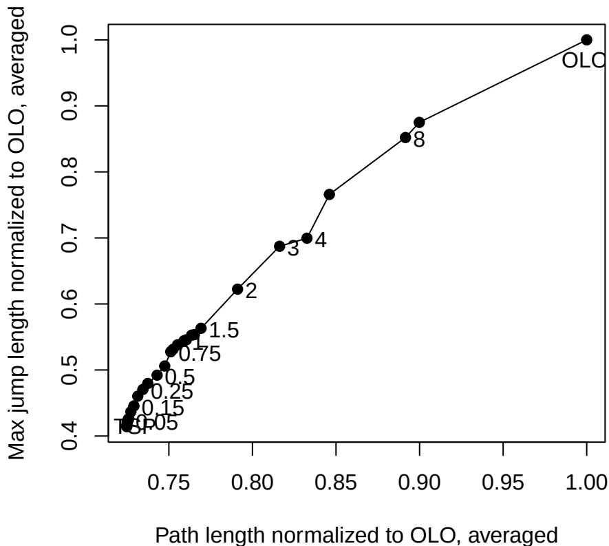
Max jump length vs PL, single linkage
