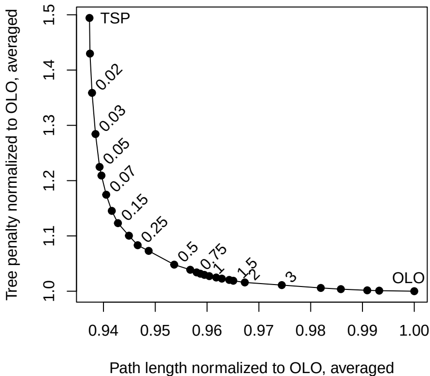
Tree penalty vs path length, ward linkage
